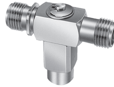
1/4" NPT or BSPT (F) inlet connection 11/16"-16 UniJet THD outlet connection
